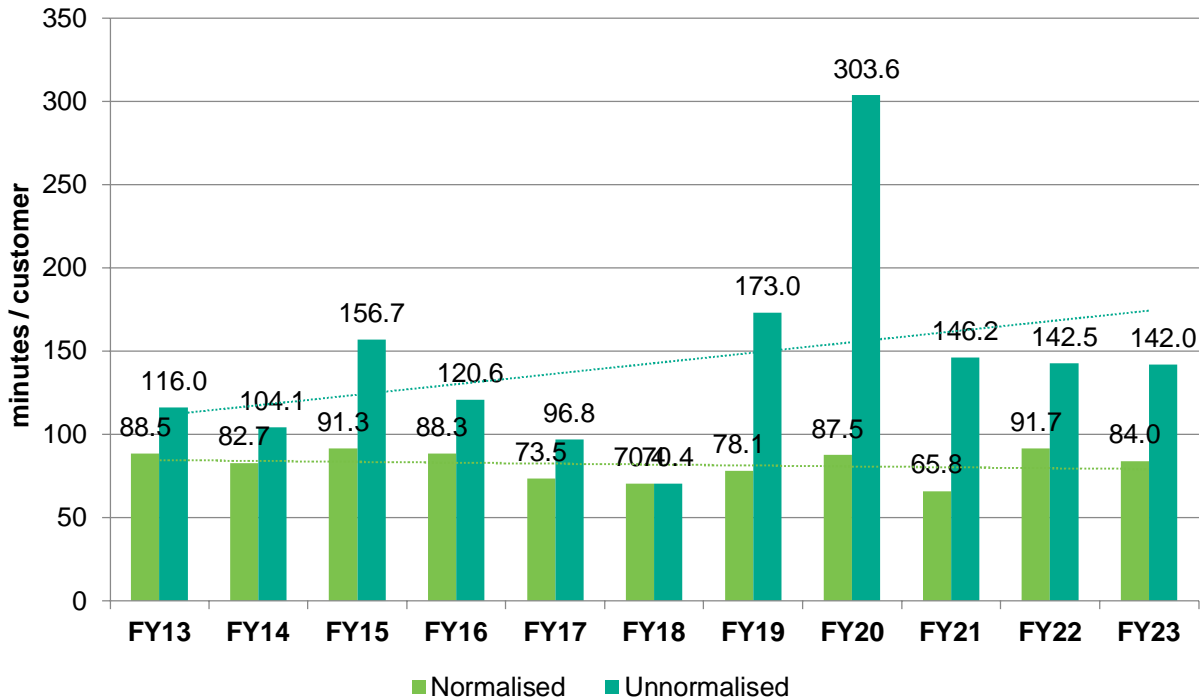
Figure 5: Organisational SAIDI Trend (Unnormalised and AER Normalised)
